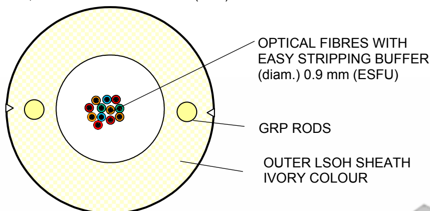
Schematic drawing not to scale (12 F version illustrated)
